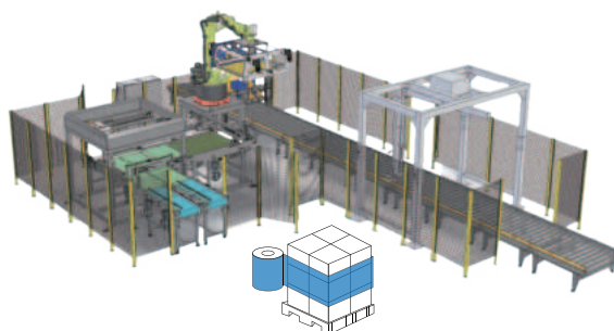
Palletizer+ Stretch Film Wrapping Machine
